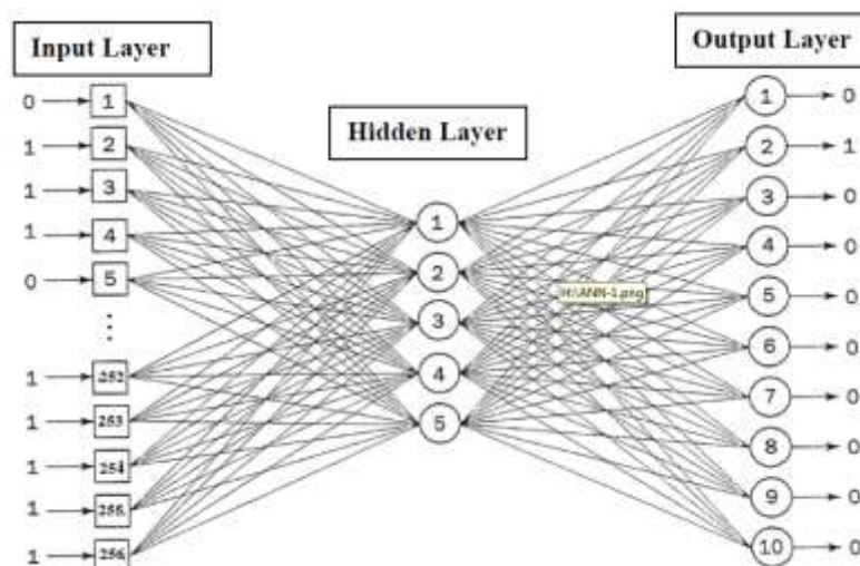
Figure 1 Architecture of Neural Network
